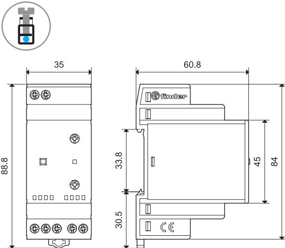
11.41 Screw terminal
