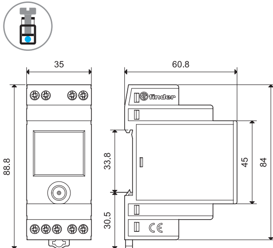
11.91 Screw terminal
